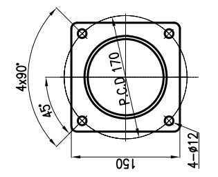
EXHAUST ELBOW FLANGE
