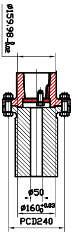
OUTPUT SHAFT COUPLING & PROPPELLER COUPLING DIMENSION
